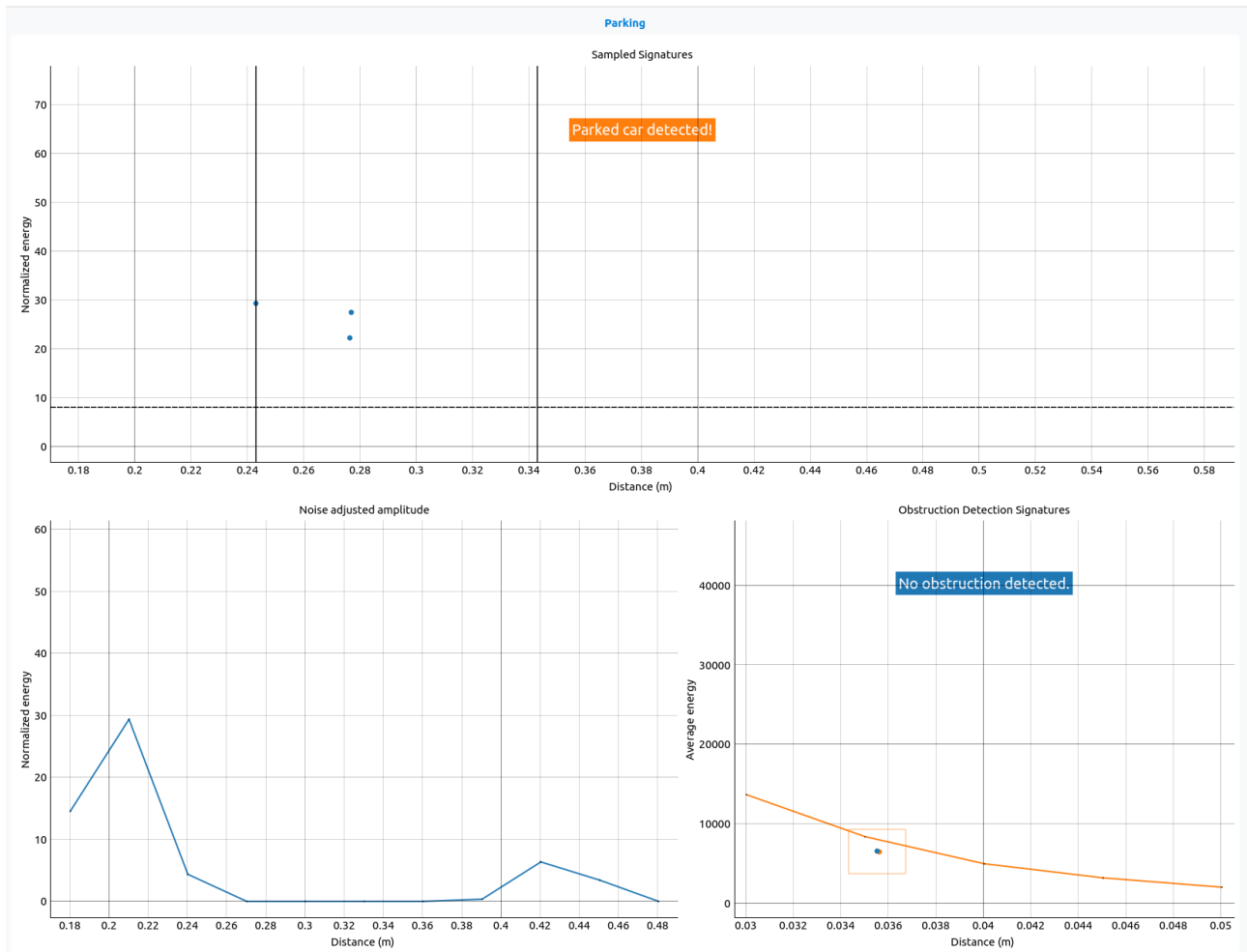
Figure 1: Example of the parking GUI with obstruction detection active. A parked car is reported and the reported object has been seen for three frames (which is indicated that you have three dots above the threshold).
