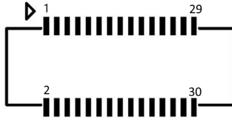
Figure 2.2. XM126 J2 connector footprint.
