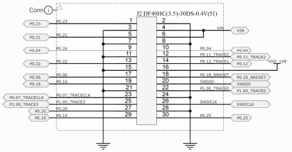
Board to board connector
