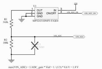
Battery voltage ADC switch
